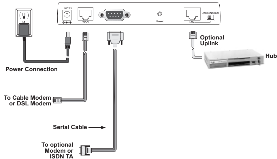
Cabling the RouteFinder RF802EW
